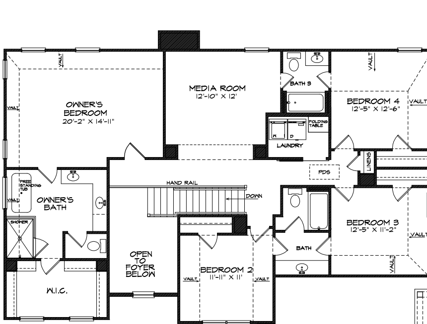
UPPER LEVEL PLAN
