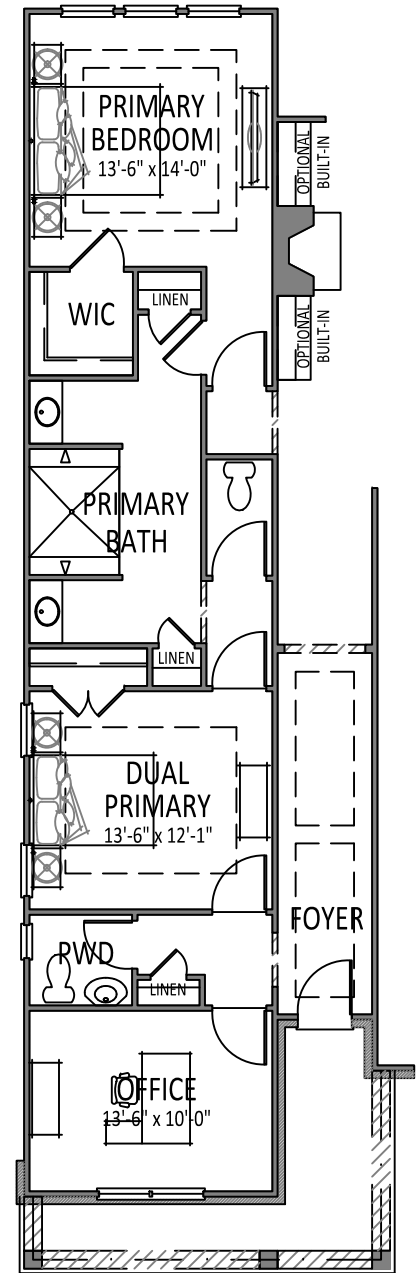
OPTIONAL DUAL PRIMARY #1
