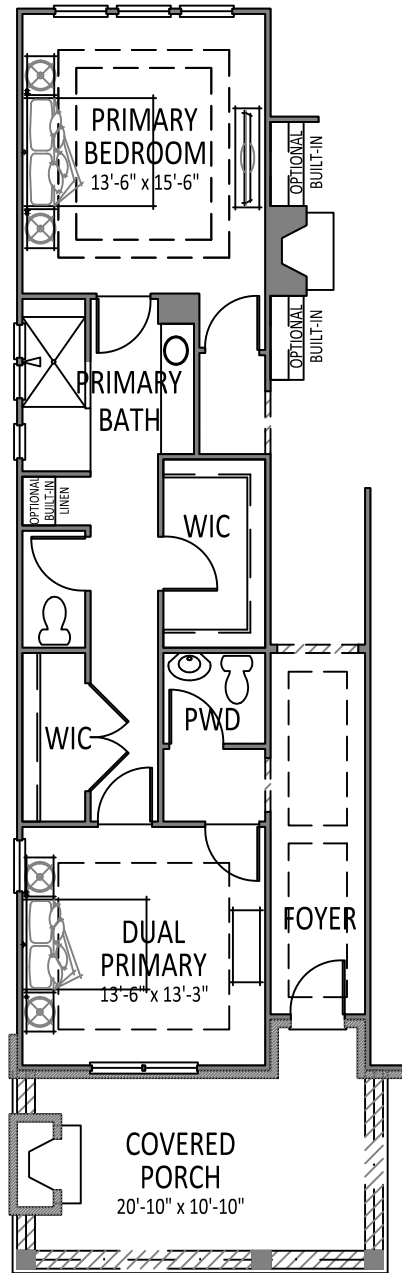
OPTIONAL DUAL PRIMARY w/ EXPANDED PORCH
