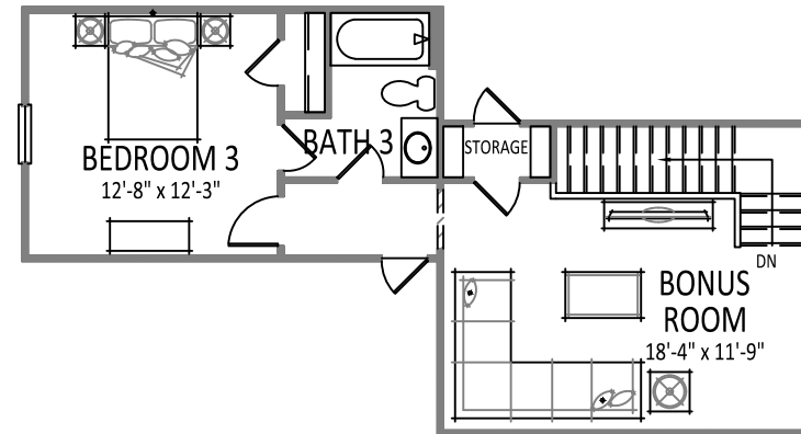
OPTIONAL 2nd FLOOR PLAN BEDROOM 3 / BATH 3 AND BONUS ROOM
