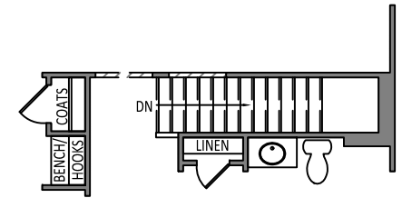
STAIRS W/ OPTIONAL BASEMENT PLAN
