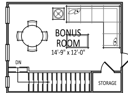
OPTIONAL 2nd FLOOR PLAN
