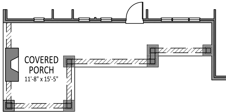
OPTIONAL EXTENDED FRONT PORCH 'C'
