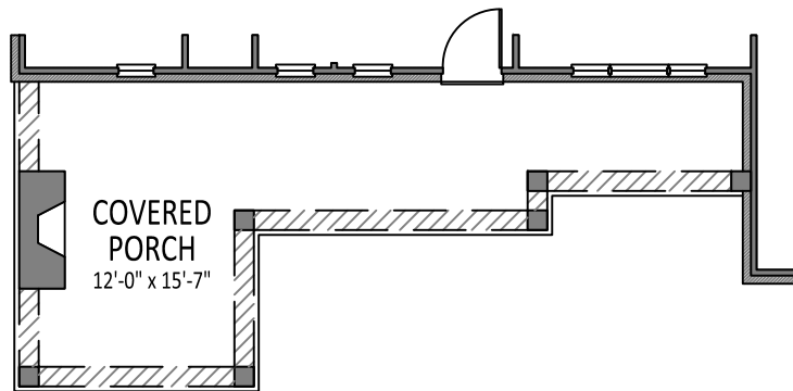
OPTIONAL EXTENDED FRONT PORCH 'B'
