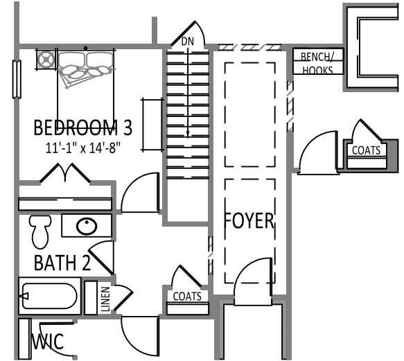
STAIRS W/ OPTIONAL BASEMENT PLAN
