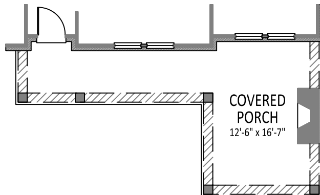
OPTIONAL EXTENDED FRONT PORCH 'A'
