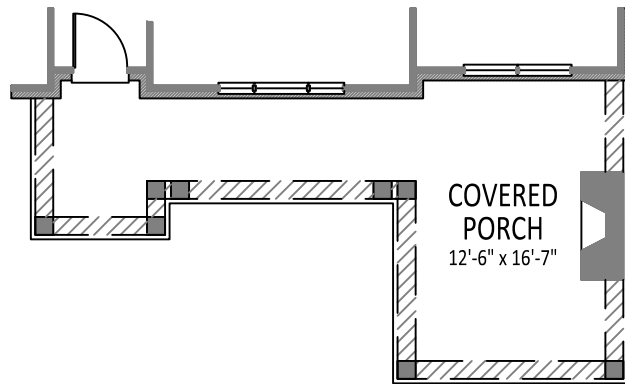
OPTIONAL EXTENDED FRONT PORCH 'B'
