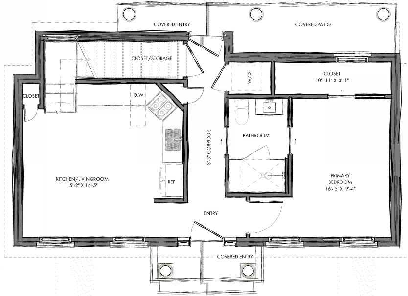
1 FLOOR PLAN 3/8" = 1'-0"
