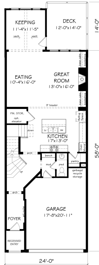
FIRST FLOOR
