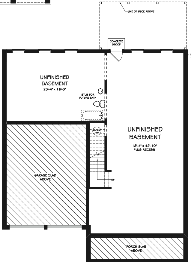
OPTIONAL GRAFTON UNFINISHED BASEMENT
