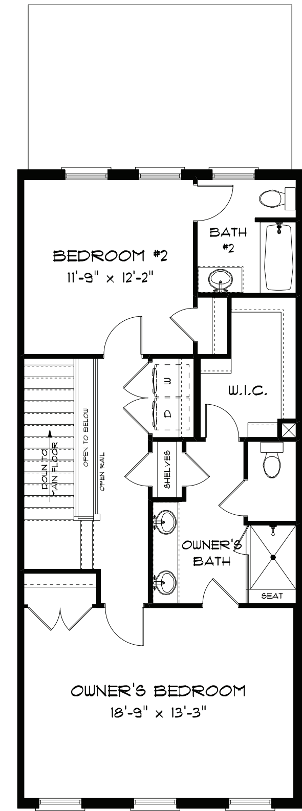
ALDER - META PLAN UPPER LEVEL INTERIOR
