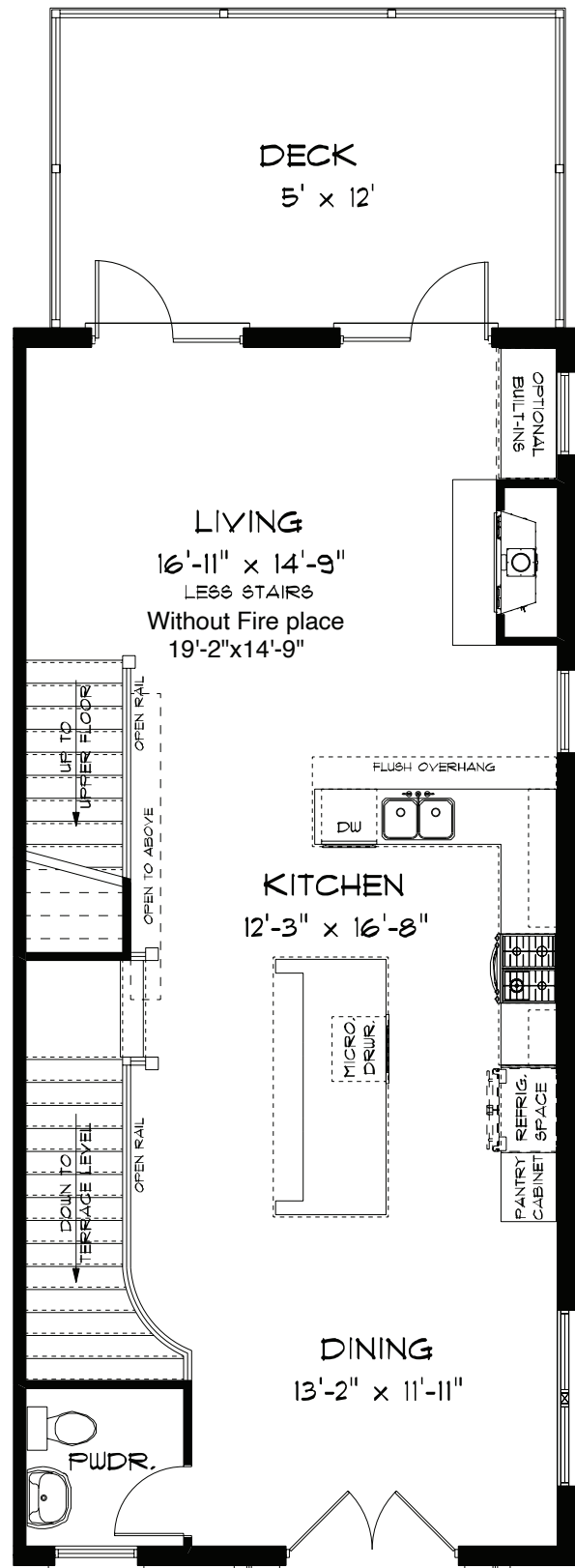
ALDER - META PLAN MAIN LEVEL EXTERIOR
