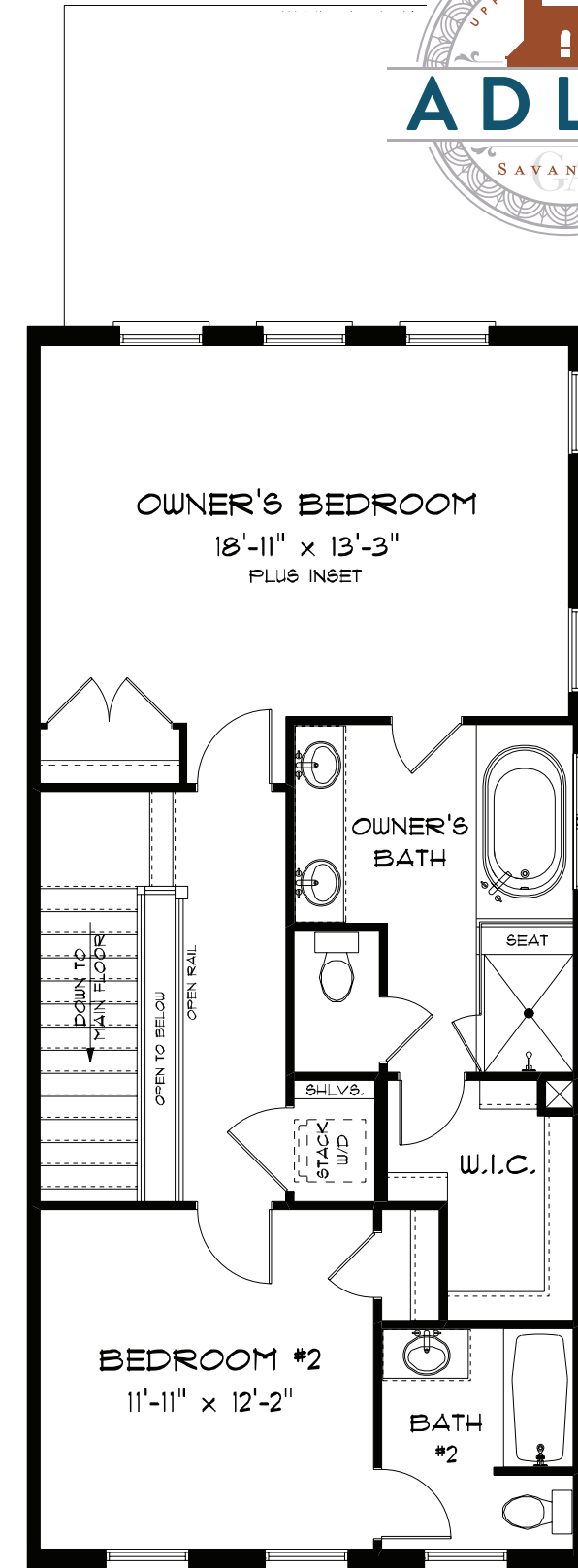
ALDER - LEE PLAN UPPER LEVEL EXTERIOR OPTIONAL TUB
