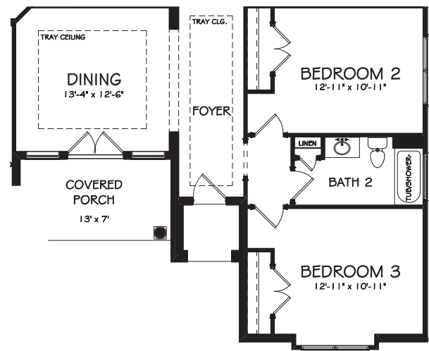
FIRST FLOOR PLAN - C
