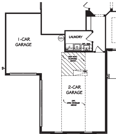
OPT. 1-CAR BOLT-ON GARAGE
