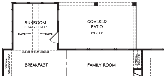
OPT. SUNROOM w/ OPT. COVERED PORCH - PLAN C
