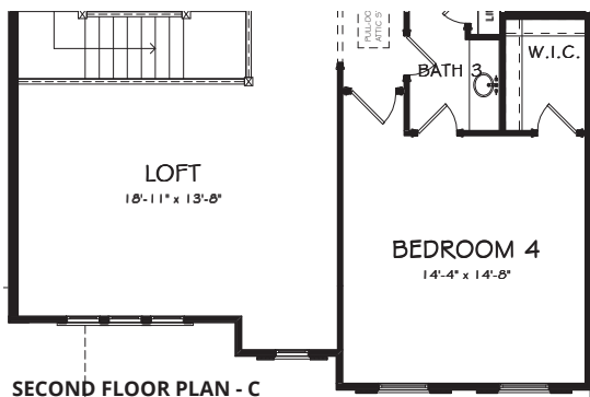
SECOND FLOOR PLAN - C
