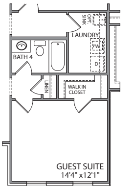
OPT. GUEST BEDROOM & BATH IN LIEU OF FLEX ROOM
