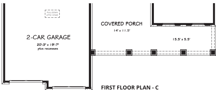
FIRST FLOOR PLAN - C
