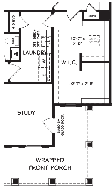
OPT. WRAPPED FRONT PORCH - PLAN C
