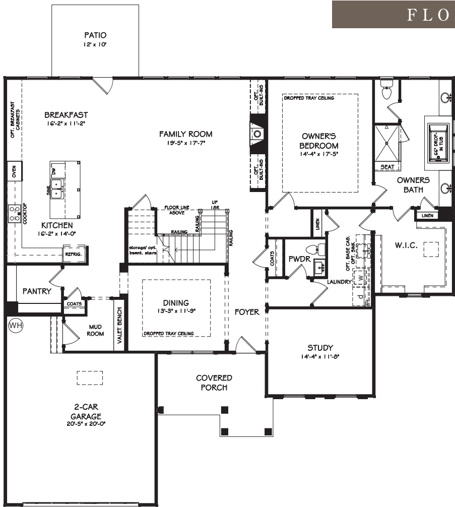
FIRST FLOOR PLAN - A&B
