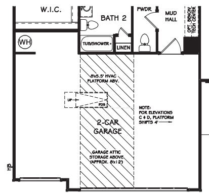
Optional Garage Attic Storage
