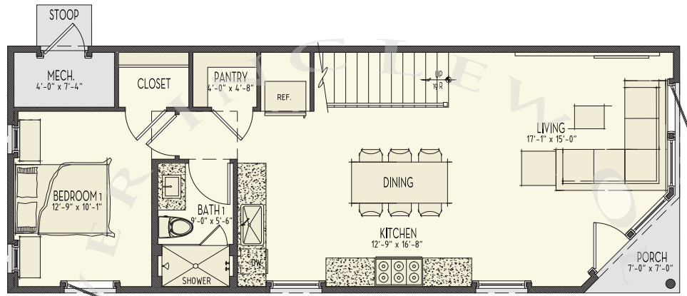
1 FIRST FLOOR PLAN SCALE: 1/4" = 1'-0"
