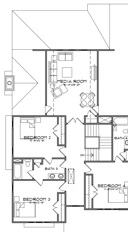
Second Level
