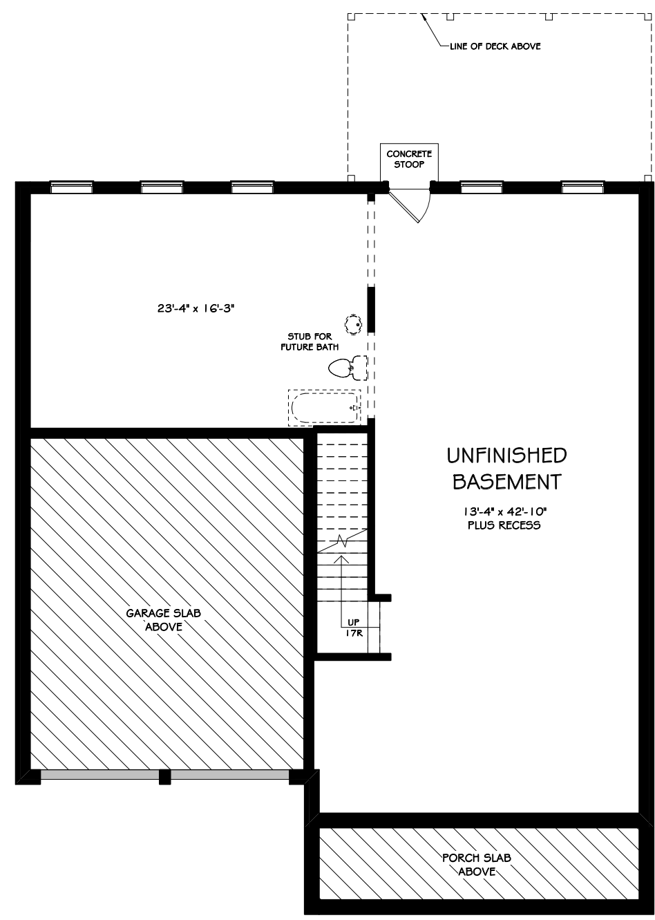
GRAFTON A BASEMENT PLAN
