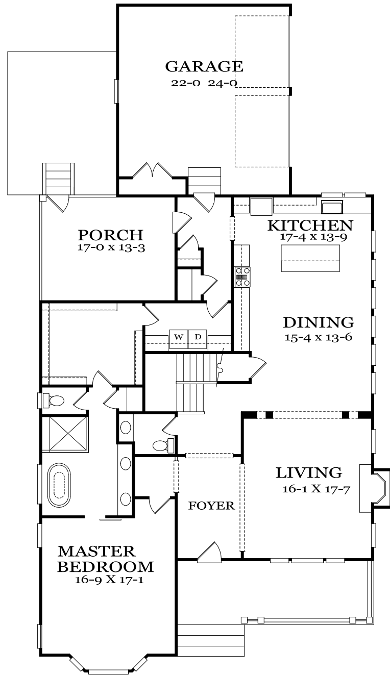
FIRST FLOOR
