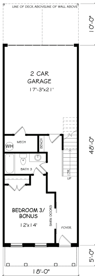
TERRACE LEVEL
