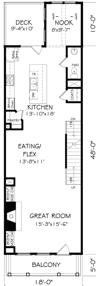
FIRST FLOOR
