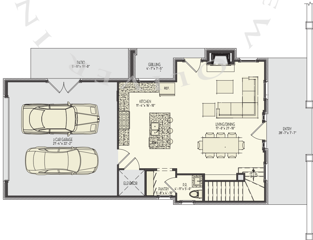
1st Floor
