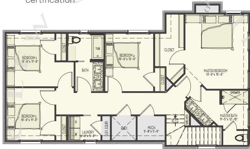
2nd Floor
