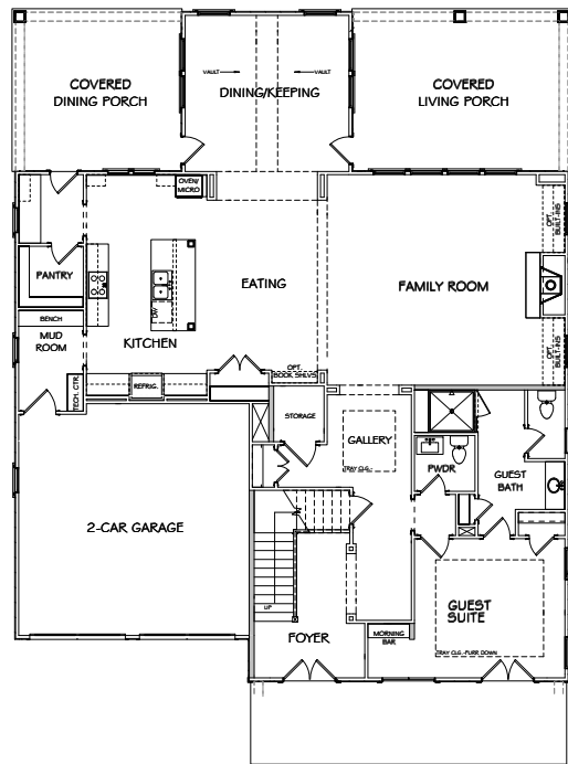
FIRST FLOOR A, B & C
