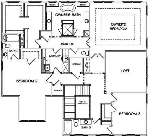
SECOND FLOOR A & C
