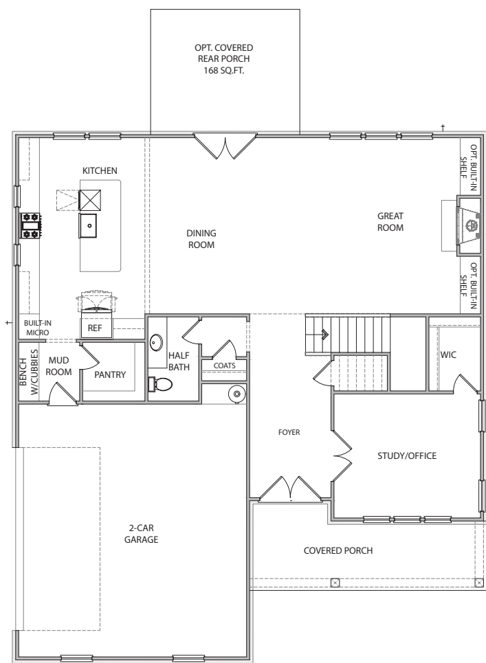
1ST FLOOR
