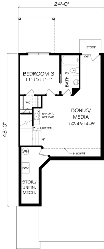
TERRACE LEVEL
