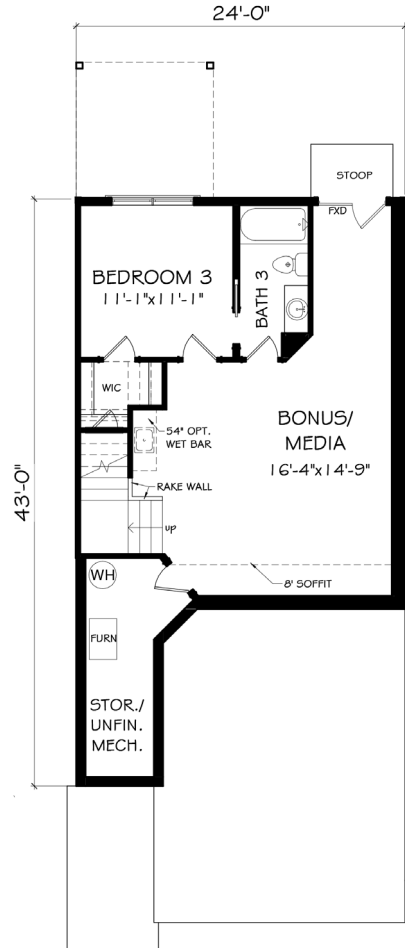
TERRACE LEVEL
