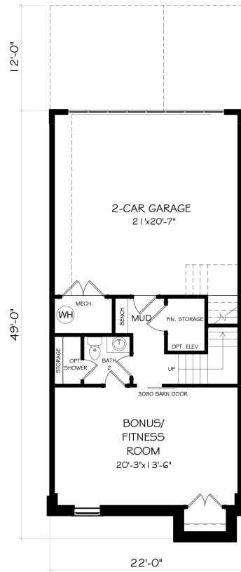
TERRACE LEVEL
