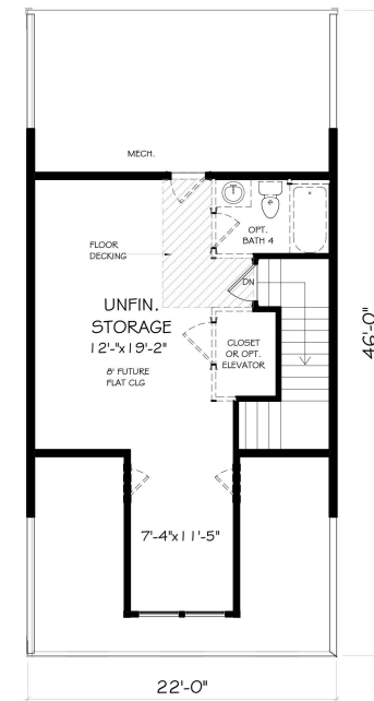
THIRD FLOOR
