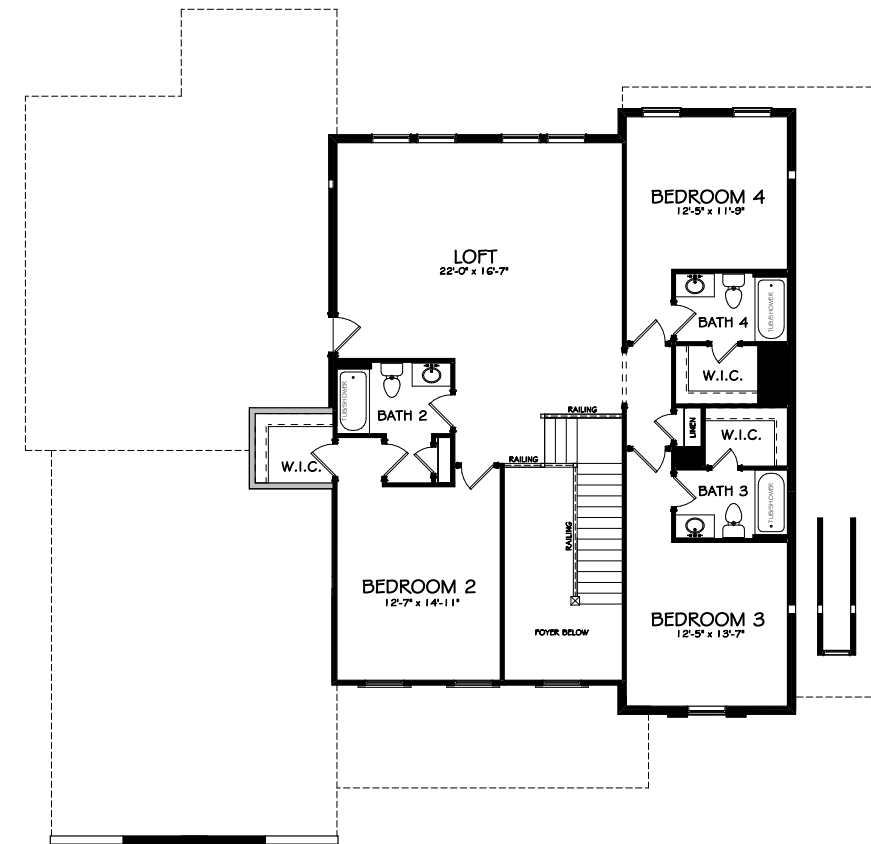
SECOND FLOOR - D
