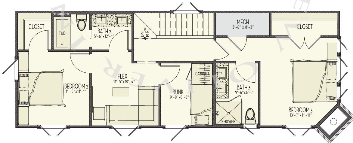
2nd Floor
