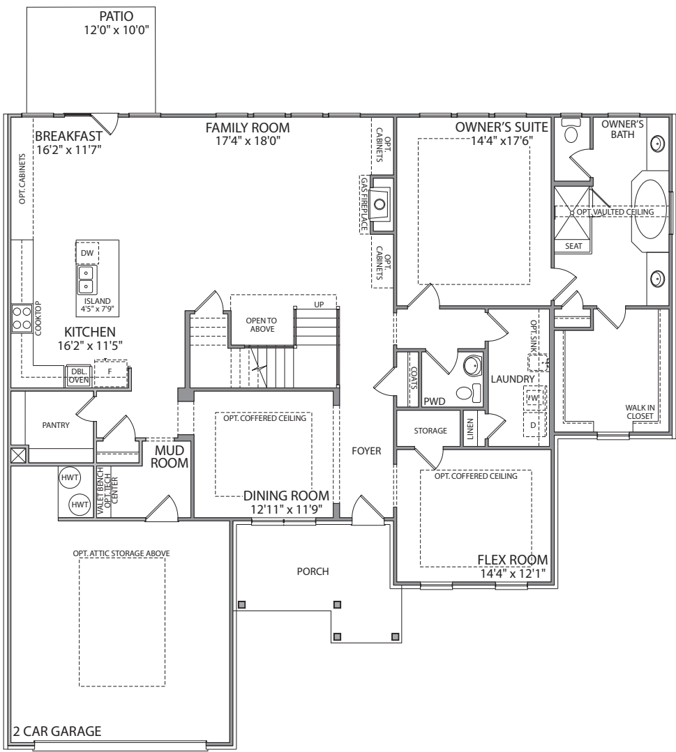
FIRST FLOOR PLAN - A&B
