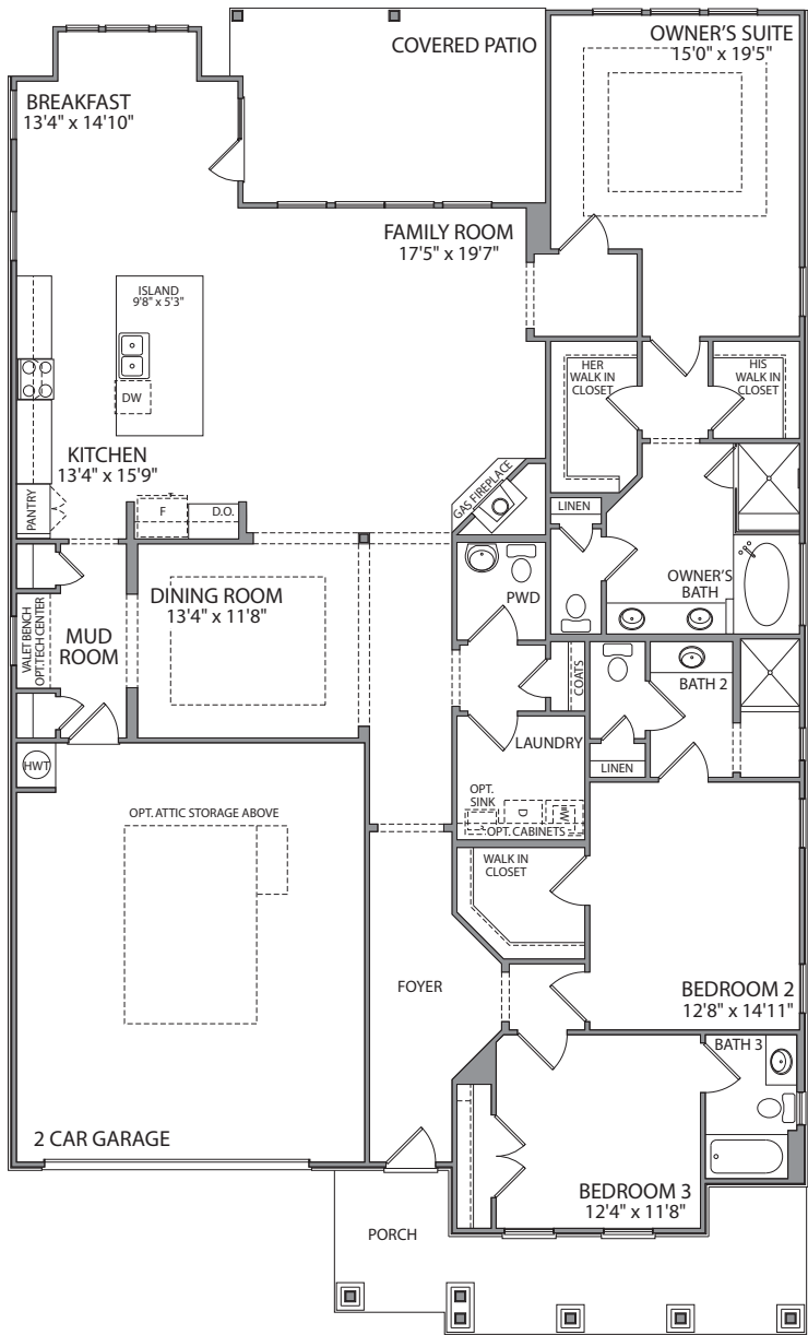
FIRST FLOOR PLAN - A
