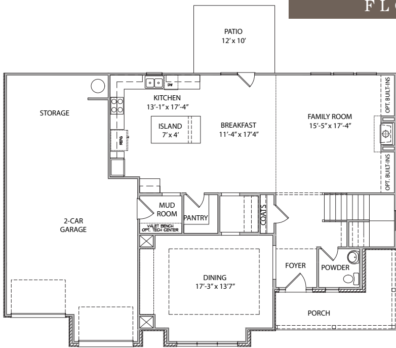
FIRST FLOOR PLAN - A
