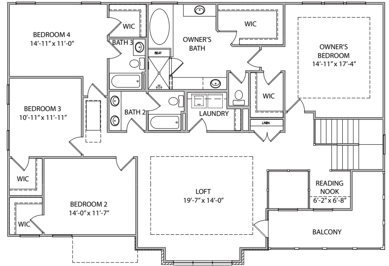
SECOND FLOOR PLAN - A
