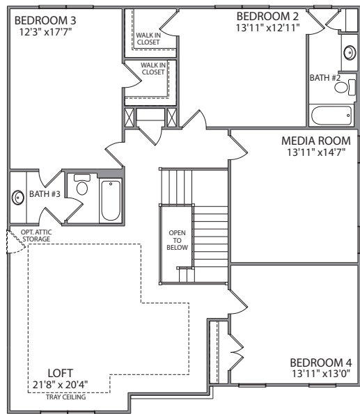
SECOND FLOOR PLAN - A
