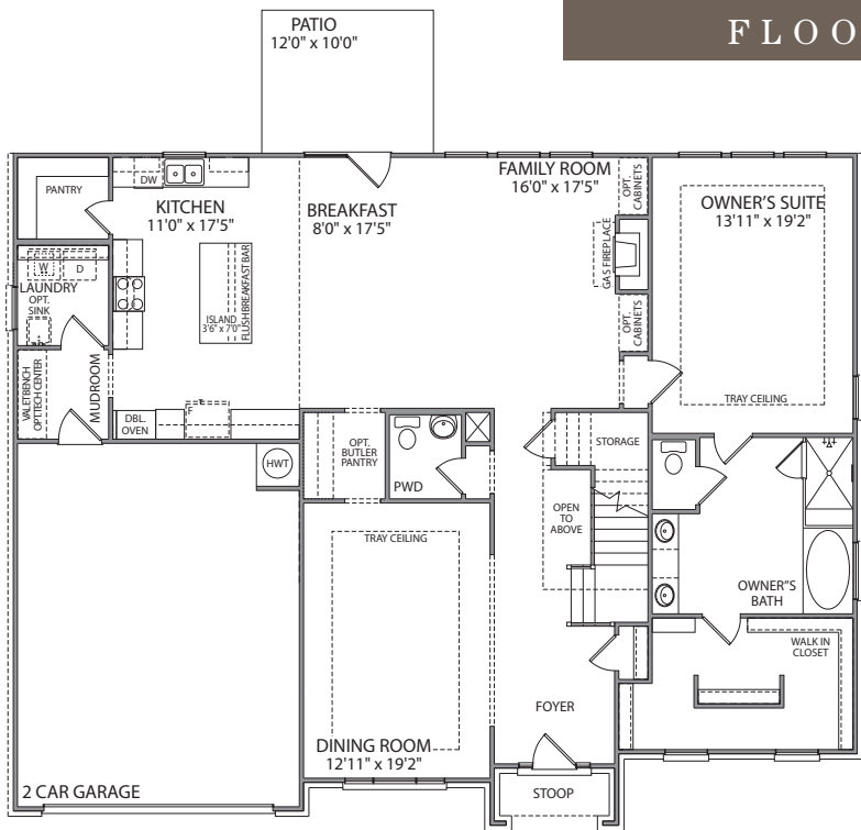
FIRST FLOOR PLAN - A
