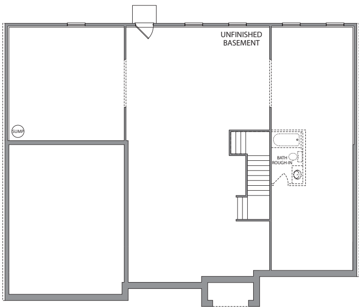
OPT. UNFINISHED BASEMENT
