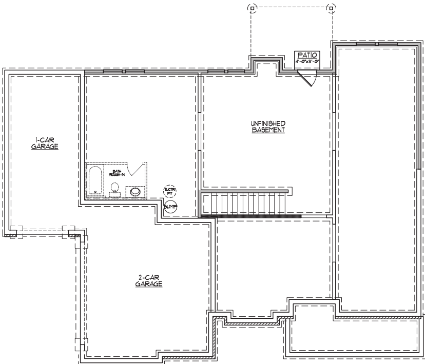
UNFINISHED BASEMENT
