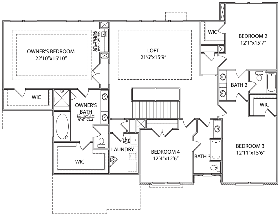
SECOND FLOOR PLAN - A
