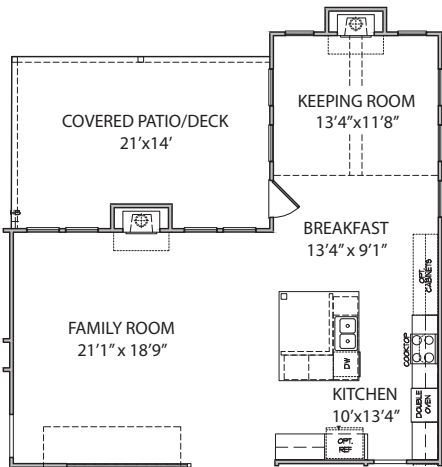
OPT. KEEPING ROOM & OPT. LARGE COVERED PATIO
