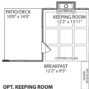
OPT. KEEPING ROOM
