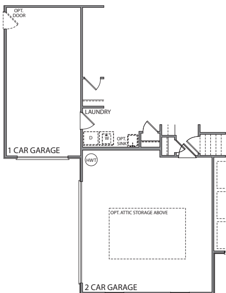
OPT. 3-CAR SIDELOAD GARAGE - A
