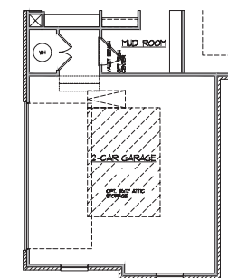
OPT. 2-CAR SIDE LOAD GARAGE
