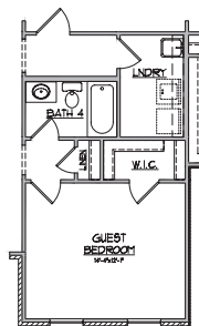
OPT. GUEST BEDROOM AND BATH ILO FLEX ROOM
