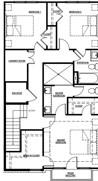
UPPER LEVEL PLAN
