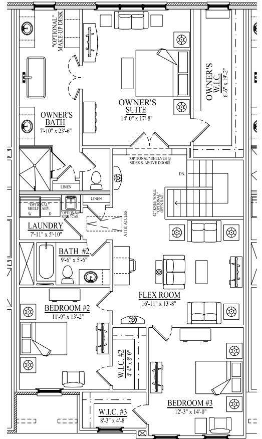
Second Floor
