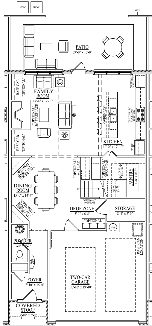
First Floor
