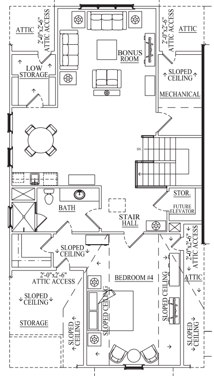
3RD FLOOR
