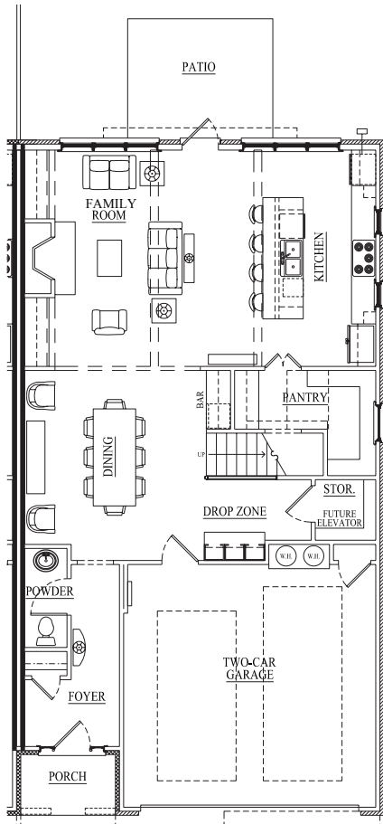
1ST FLOOR
