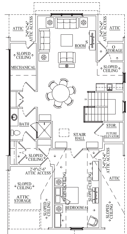
3RD FLOOR
