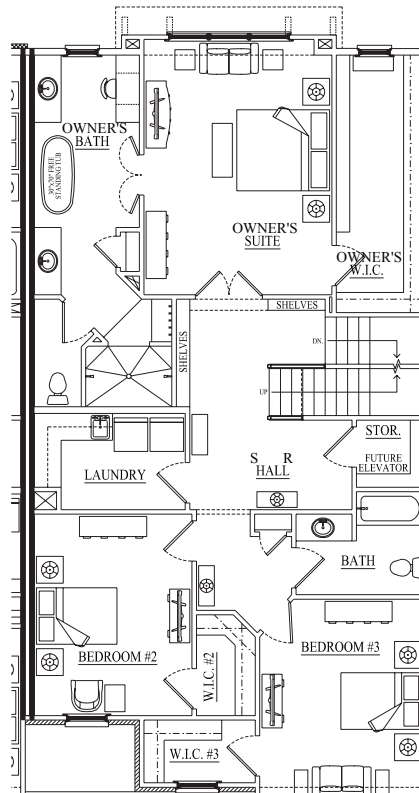
2ND FLOOR
