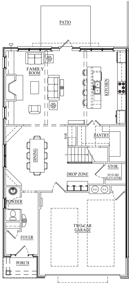
1ST FLOOR
