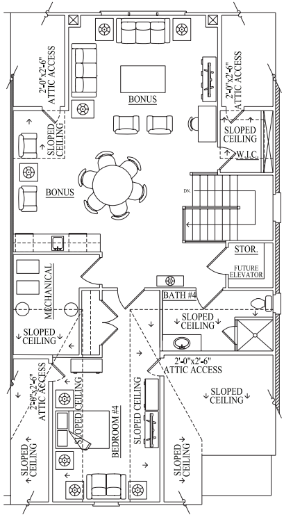
3RD FLOOR
