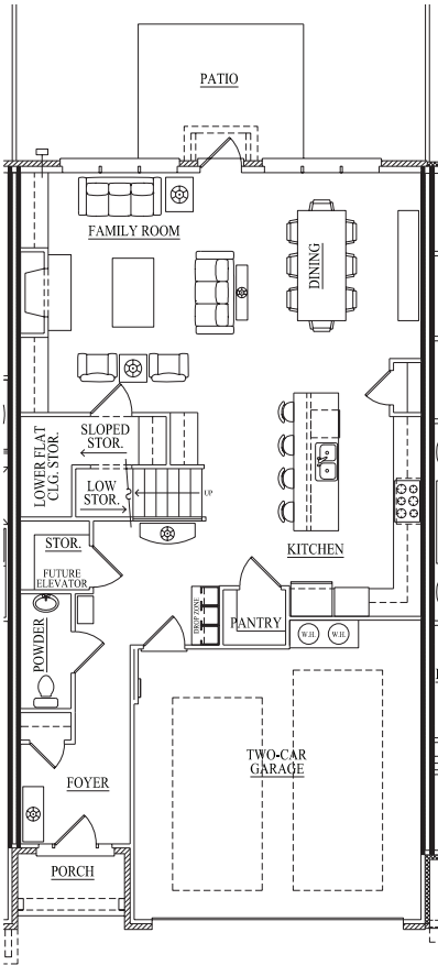
1ST FLOOR
