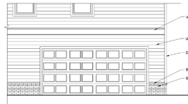
OPTIONAL SIDE ENTRY GARAGE - ELEVATION
