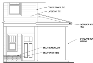
EXTENDED REAR PORCH REAR ELEVATION
