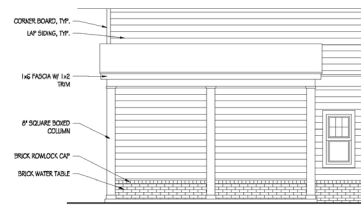
EXTENDED REAR PORCH SIDE ELEVATION
