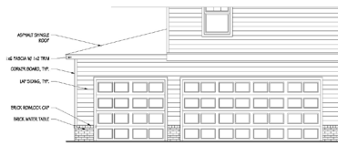
3-CAR GARAGE REAR ELEVATION
