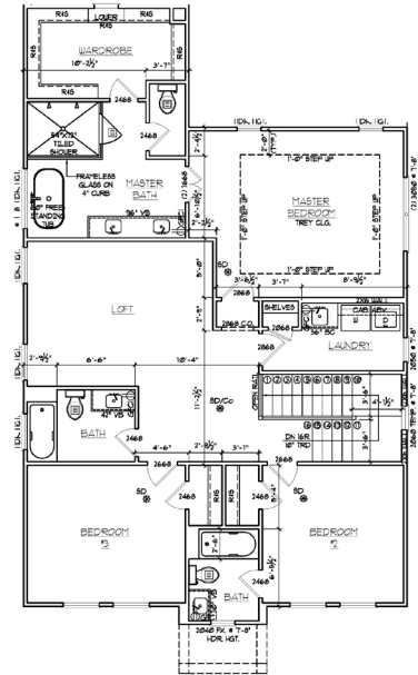
Second Floor with Opt. Loft
