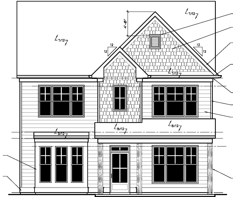
Elevation C
