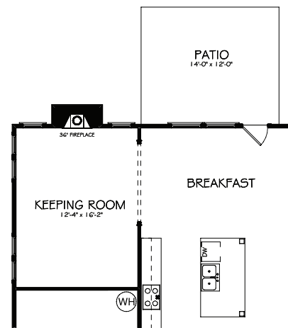
OPTIONAL KEEPING ROOM AND PATIO
