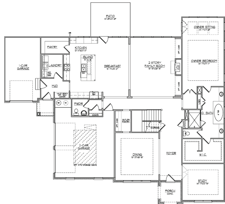
FIRST FLOOR - A
