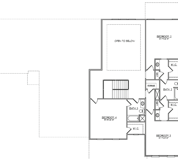
SECOND FLOOR - B
