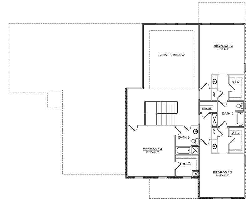
SECOND FLOOR - C
