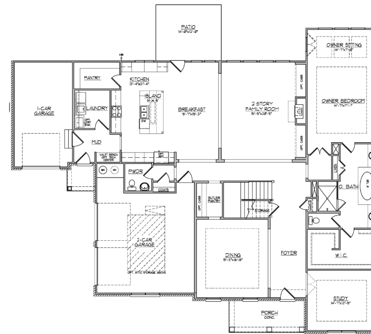
FIRST FLOOR - C
