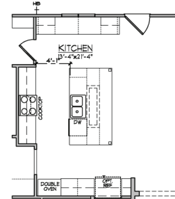
OPTIONAL DELUXE KITCHEN
