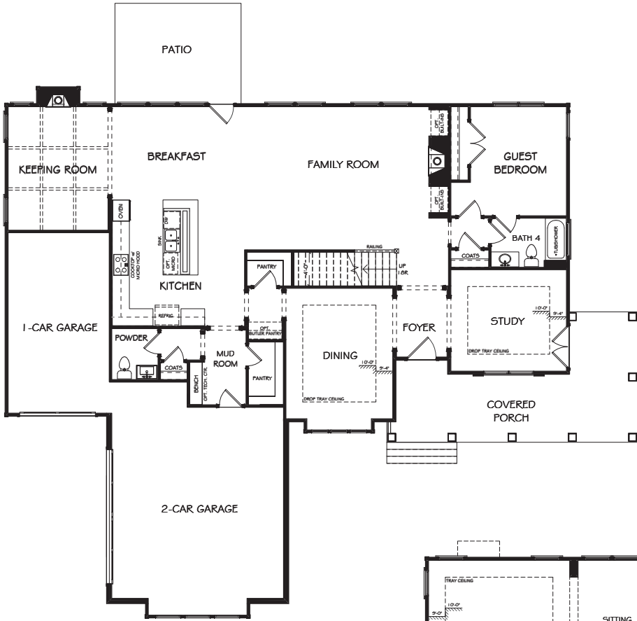
FIRST FLOOR PLAN - G
