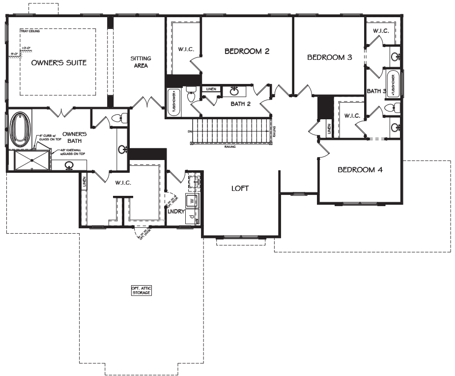
SECOND FLOOR PLAN - G
