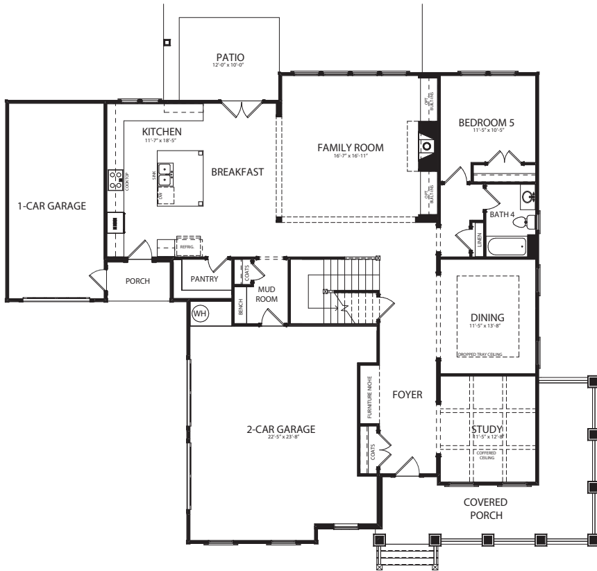
FIRST FLOOR PLAN - G
