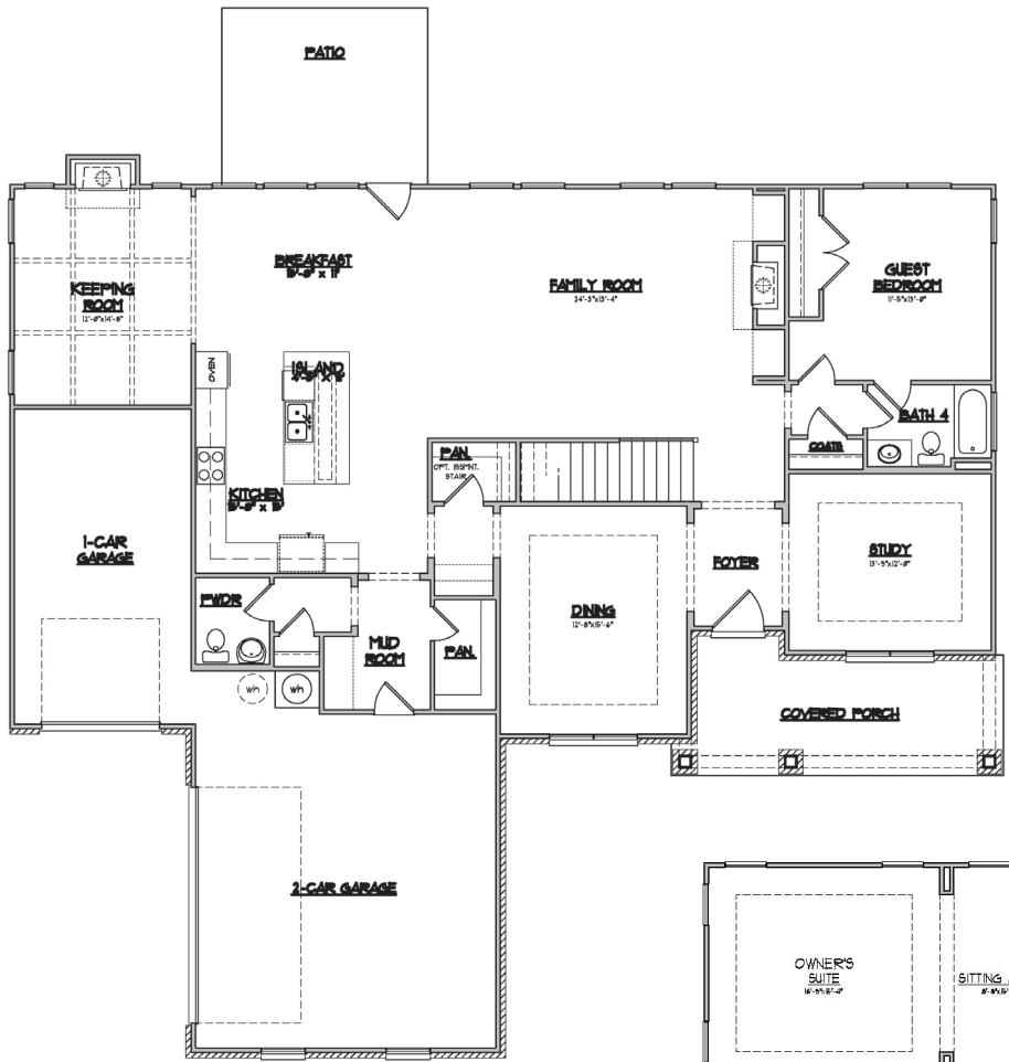
FIRST FLOOR - A
