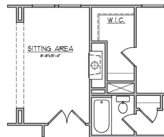
OPTIONAL NAPOLEAN FIREPLACE IN OWNER SITTING
