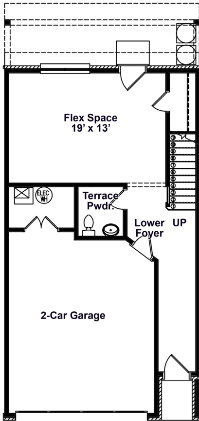
Lower Level
