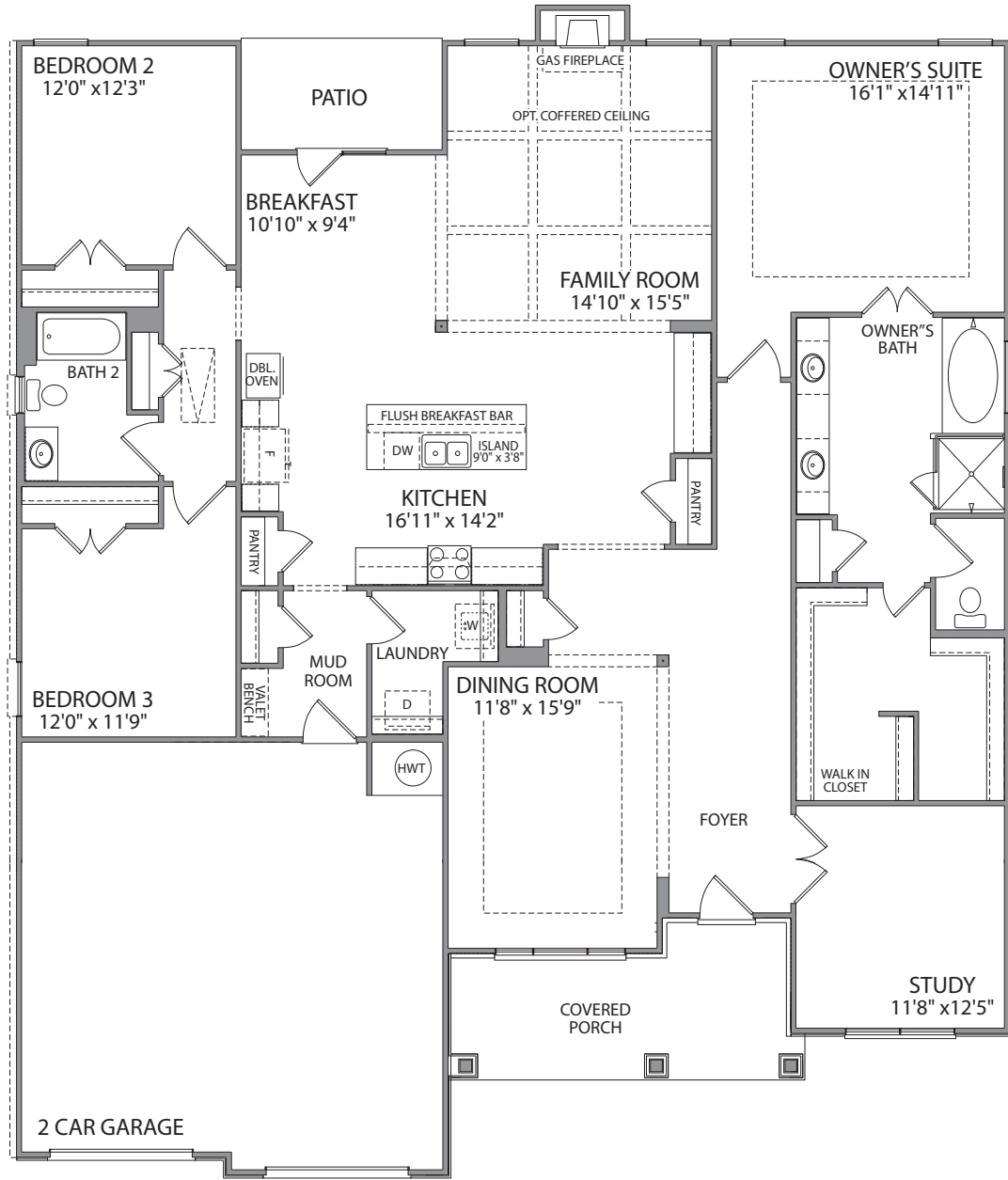
FIRST FLOOR ELEV. D
