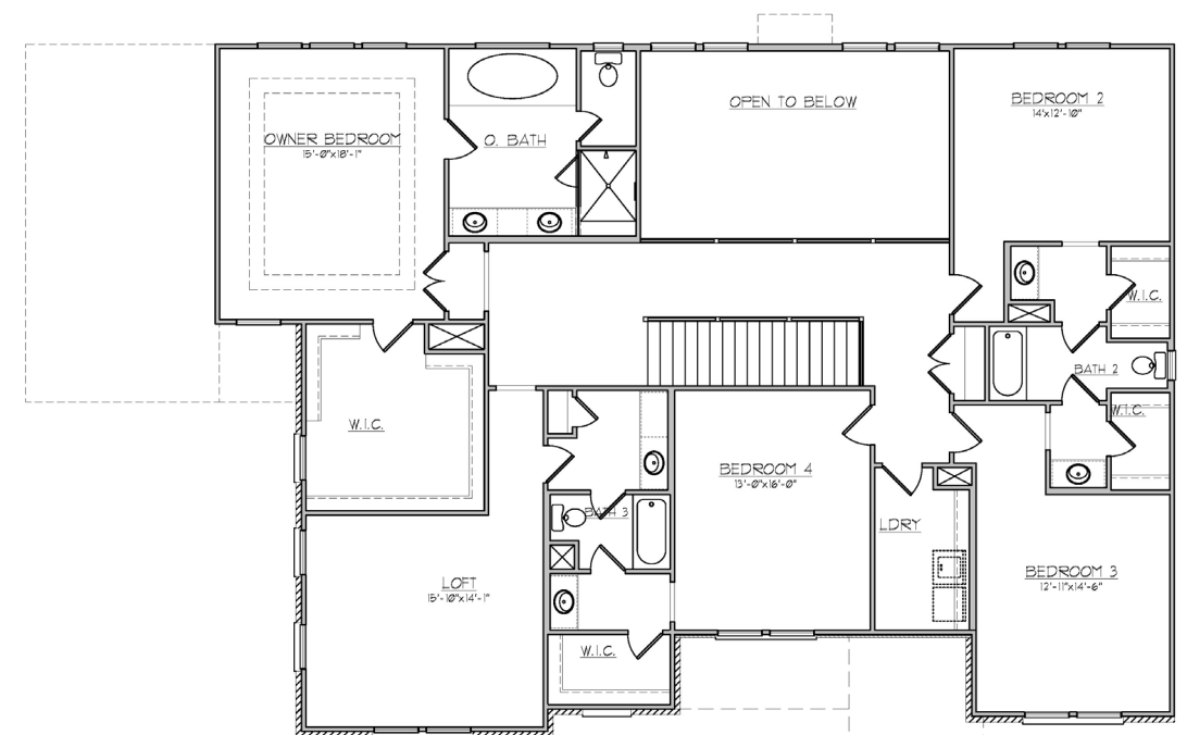
SECOND FLOOR - B
