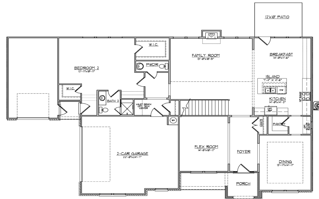
FIRST FLOOR - B
