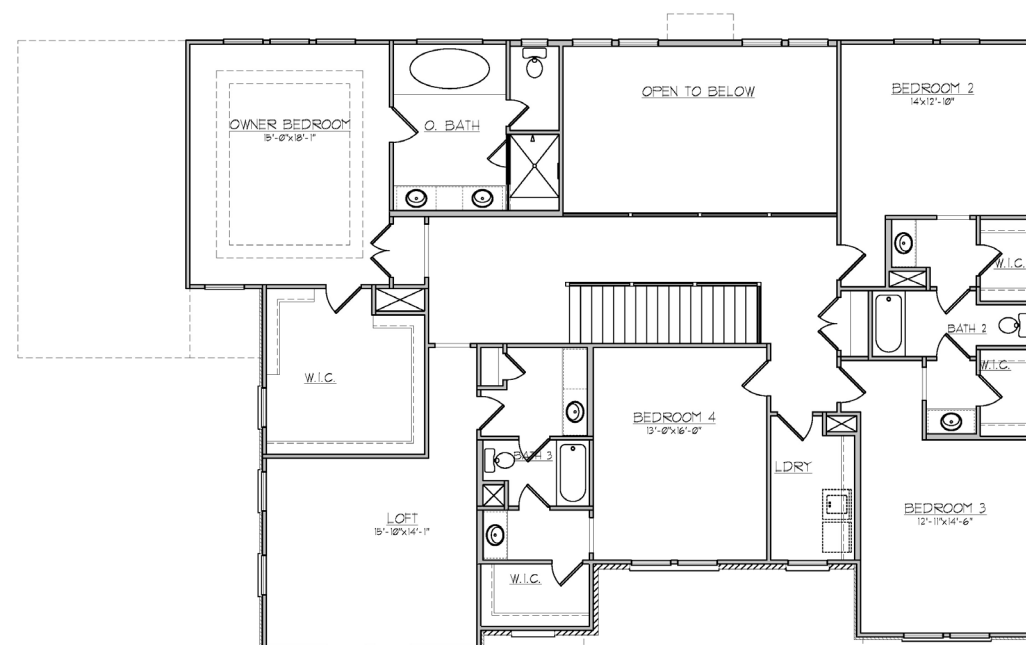
SECOND FLOOR - A
