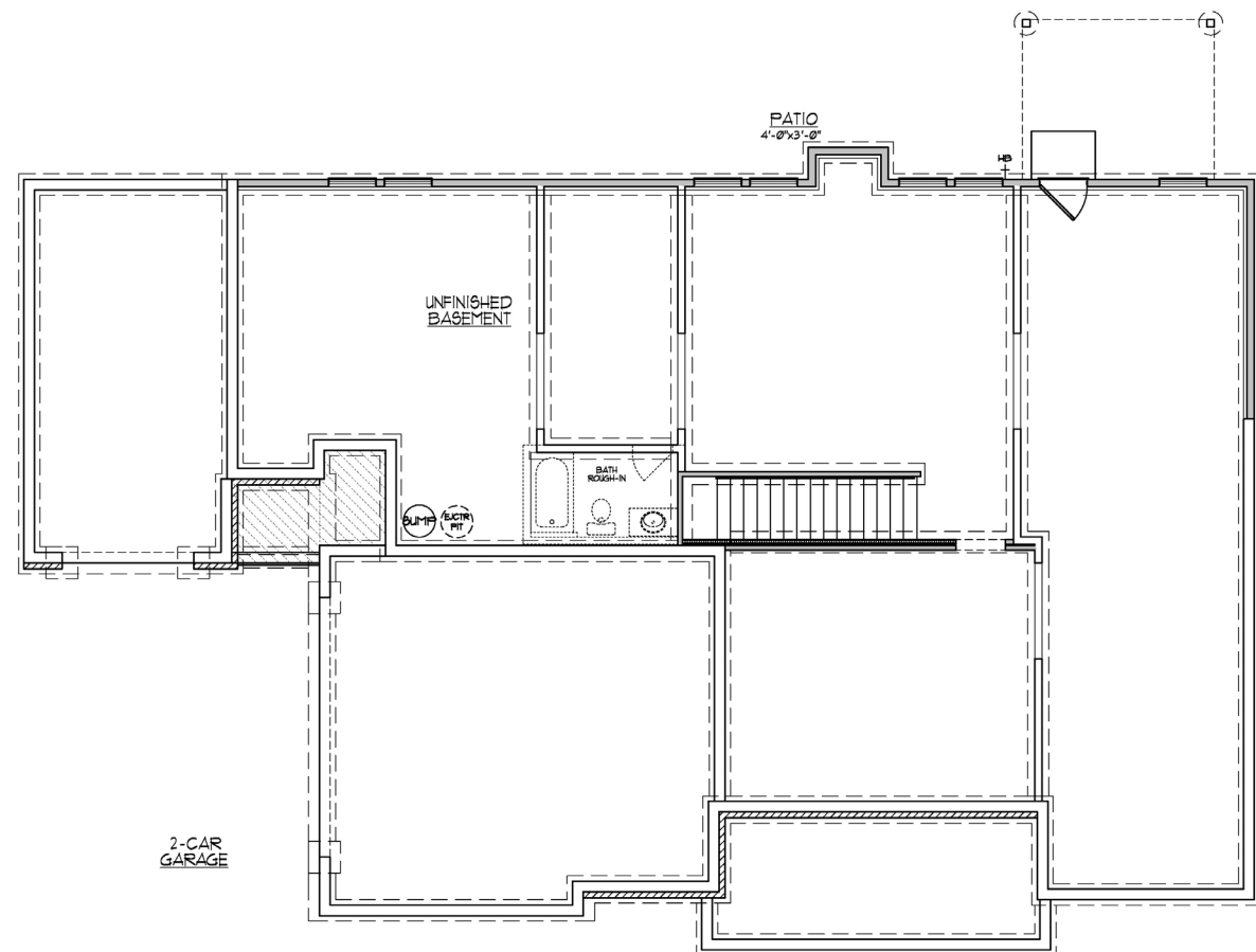
UNFINISHED BASEMENT - PLAN A
